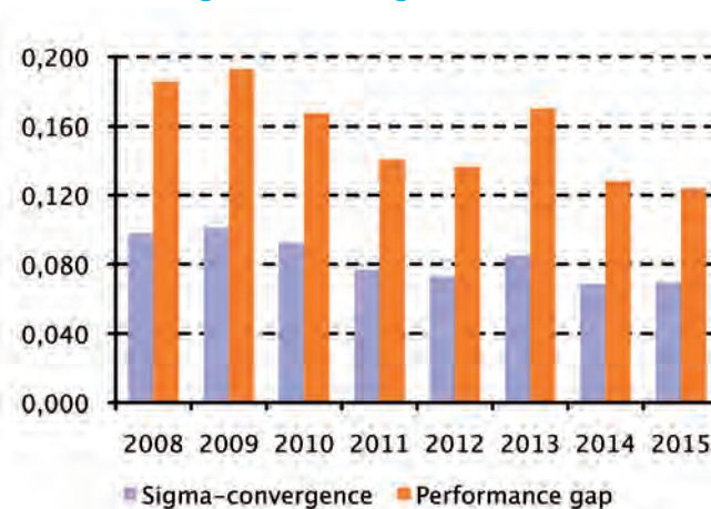
Figure 12: Strong Innovators
