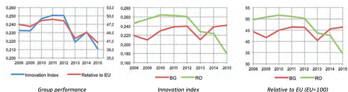
Figure 7: Modest Innovators
