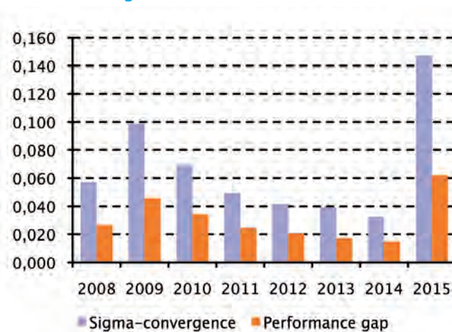
Figure 14: Modest Innovators
