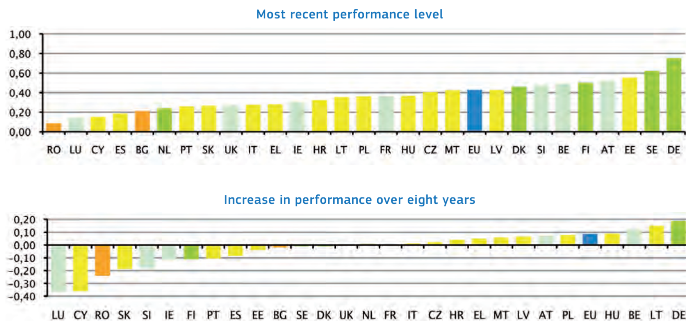
Figure 19: Firm investments
